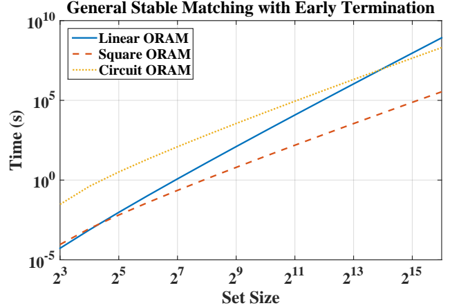
Fig. 8. Total running time of the GC protocol using different ORAM schemes for general SM using early termination technique.
