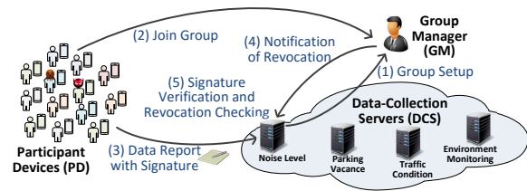
Fig. 1. System Overview of GROUPSENSE
