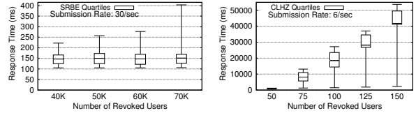
(a) SRBE scheme
