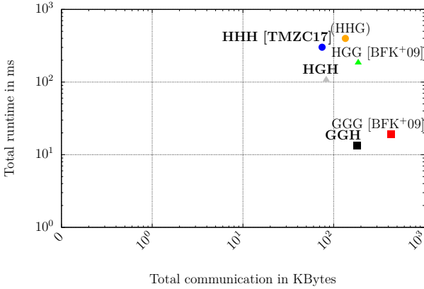
(a) Tradeoff for small dataset wine.
