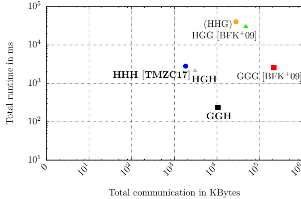
(b) Tradeoff for large dataset boston.
