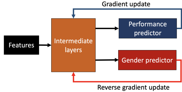
Fig. 2. Schematic diagram of the proposed model. Parameters in the intermediate layers are updated along the gradient sent by the ‘performance predictor,’ but along the opposite direction of the gradient sent by the ‘gender predictor.’ Thus, gender information is censored from the intermediate representation of the input features.
